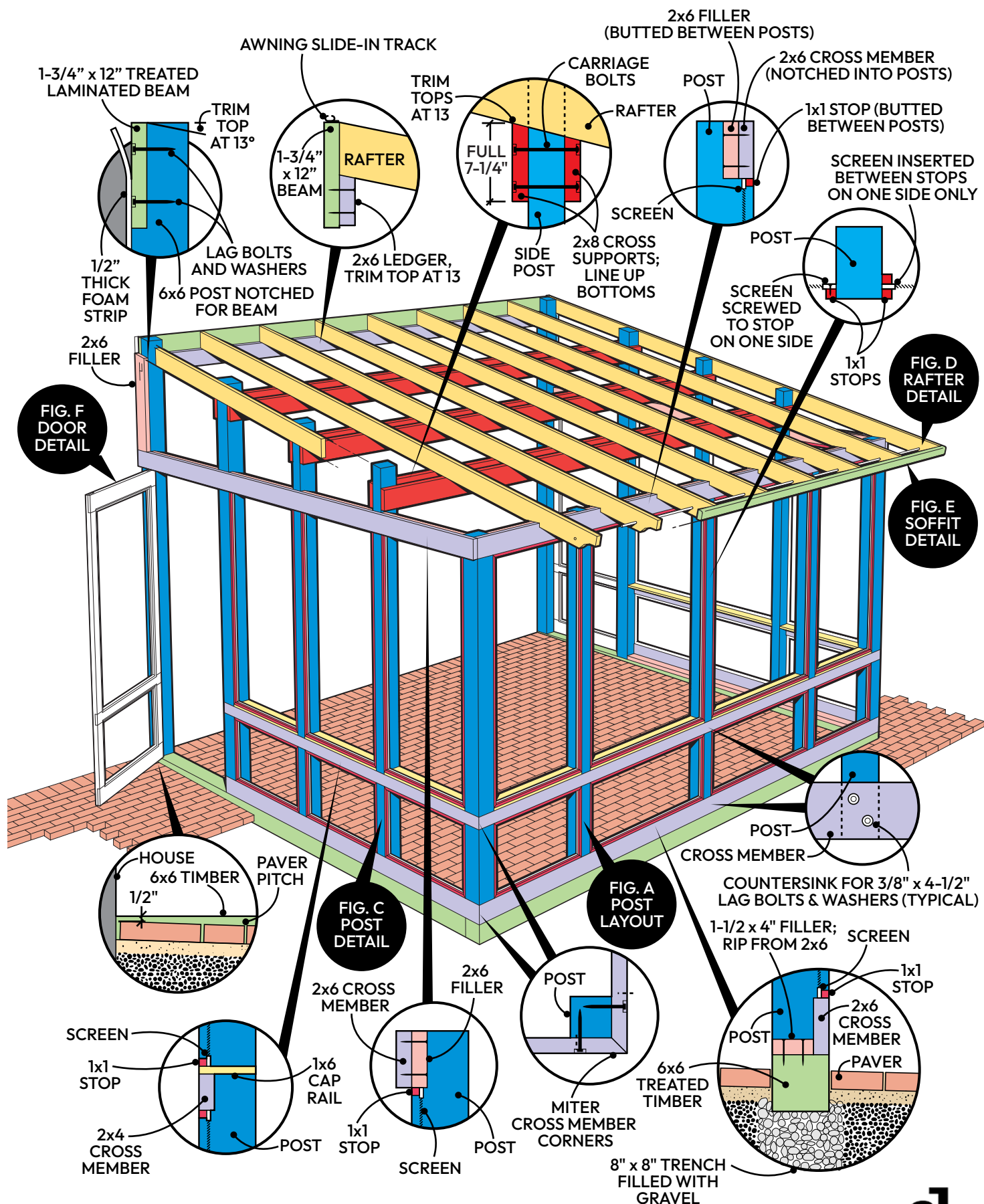
FIG. B SCREENED PATIO OVERVIEW
